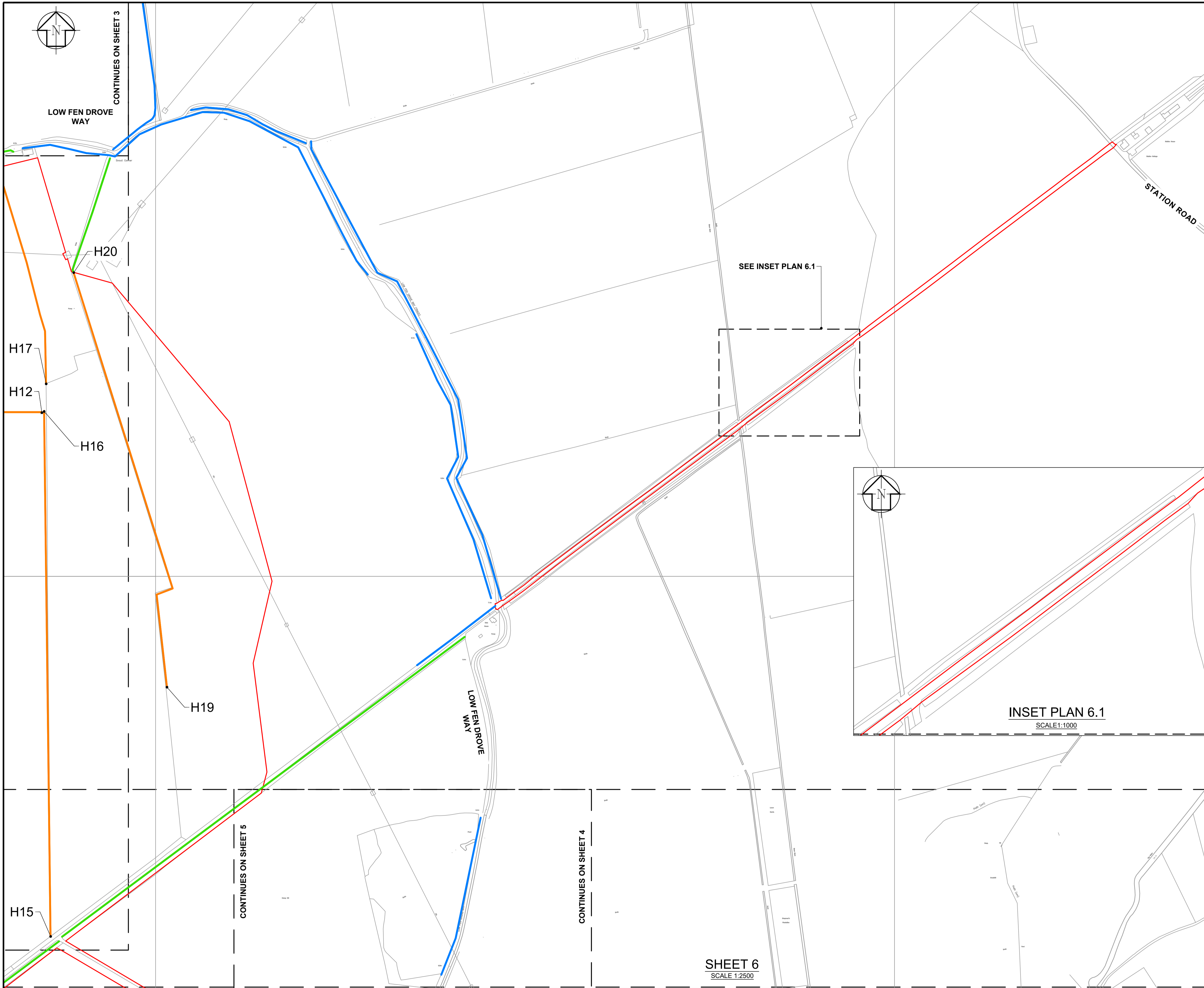
SCALE 1:2500 0m 25m 50m 75m 100m SCALE 1:1000 0m 10m 20m 30m 40m 50m
